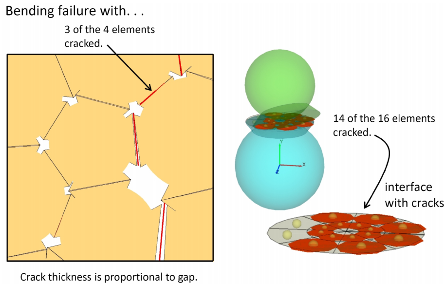
Figure 12 Partially damaged flat-jointed material showing faced grains with cracks colored red/blue for tensile/shear failure. (From Fig. 3 of Itasca [2019] 22 .)
