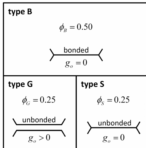
Figure 13 Initial microstructure of flat-jointed material: each flat-joint contact is bonded (type B), gapped (type G) or slit (type S).
