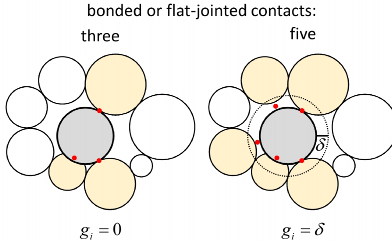
Figure 26 Grain assembly at end of packing phase with the bonded or flat-jointed contacts of a typical grain when the installation gap is zero (left) and greater than zero (right). Increasing the installation gap increases the grain connectivity.
