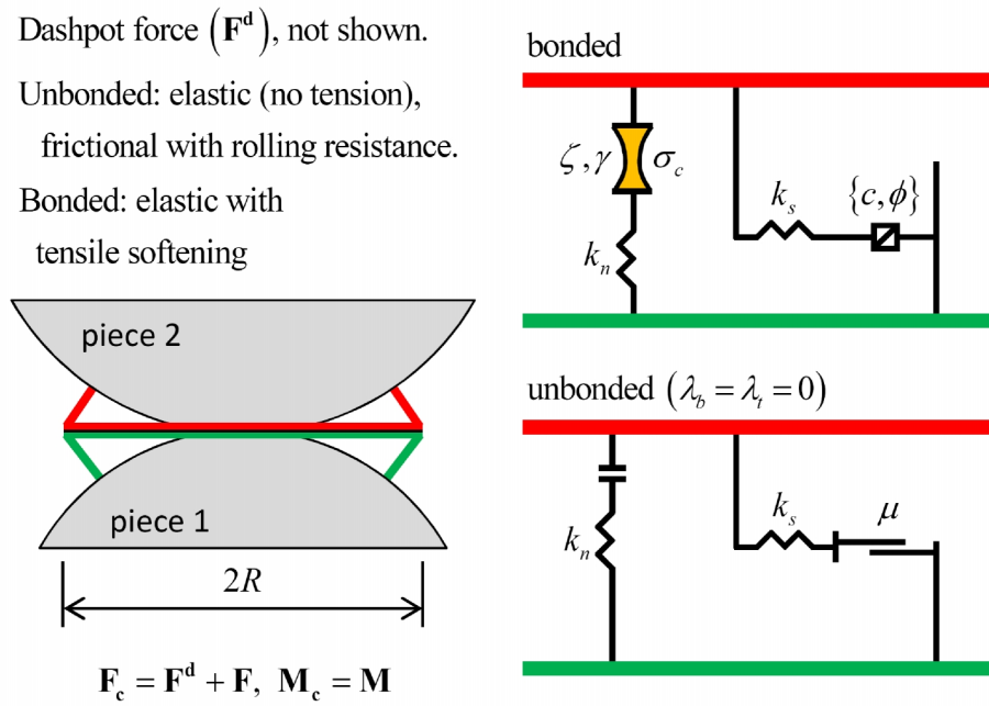
Figure 7 Behavior and rheological components of the soft bond model with friction multipliers of zero and inactive dashpots.
