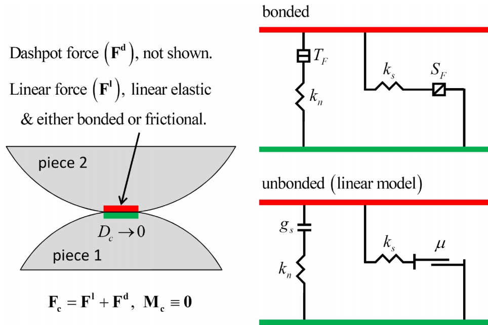
Figure 5 Behavior and rheological components of the linear contact bond model with inactive dashpots. (From Fig. 1 of Itasca [2019] 13 .)
