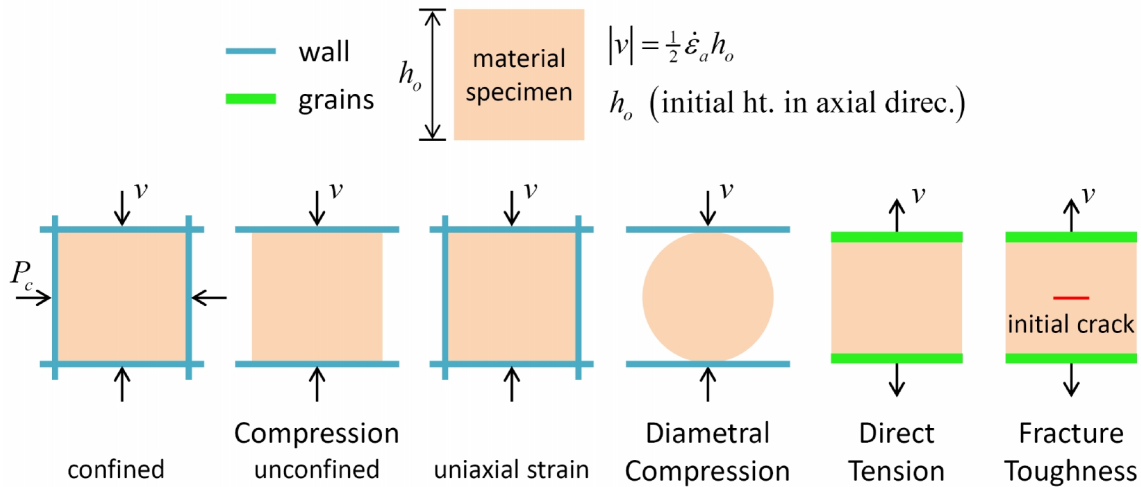
Figure 29 Loading conditions of laboratory-testing procedures.
