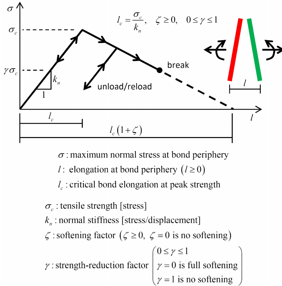
Figure 8 Softening behavior of the soft bond model.
