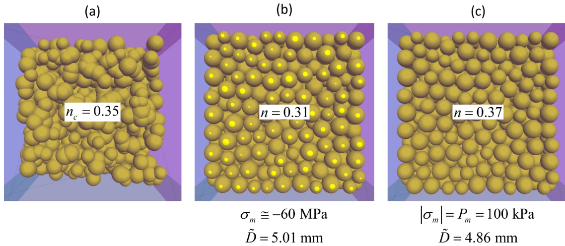
Figure 25 Grain-scaling packing procedure: (a) initial grain cloud at end of step 1, (b) relaxed grain cloud at end of step 2, and (c) compacted granular assembly at end of step 3. The images show the SS_ContactBonded material of the contact-bonded material example.
