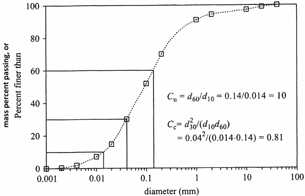
Figure 15 Typical grain size distribution curve showing the cumulative distribution of mass according to particle size. (From Fig. 2.10 of Santamarina et al. [2001].)
