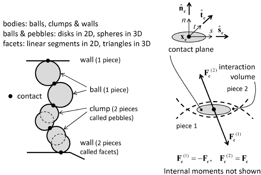
Figure 1 PFC model showing bodies and contacts (left) and contact plane with internal force (right). (From Fig. 1 of Itasca [2019] 7 .)
