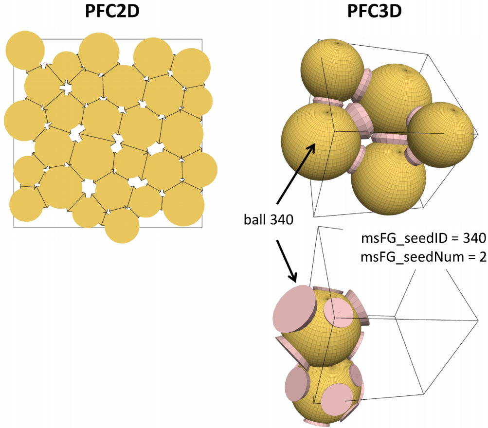
Figure 18 Faced grain plot set showing faced grains in the microstructural box (top) and connected to a seed grain (bottom).
