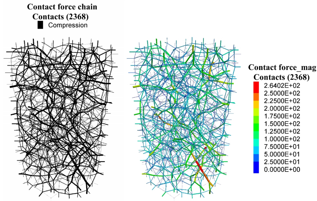
Figure 21 Force-chain fabric in the linear material packed at 150 kPa material pressure showing: bi-colored (left) and scale-colored (right) displays. The linear material cannot sustain tension, therefore the bi-colored display shows only compression.
