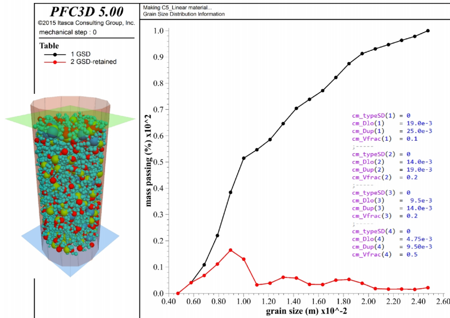
Figure 16 Grain size distribution information produced by the FISH function gsdMeasure(19) showing cumulative mass percent passing (in black) and incremental mass percent retained (in red).
