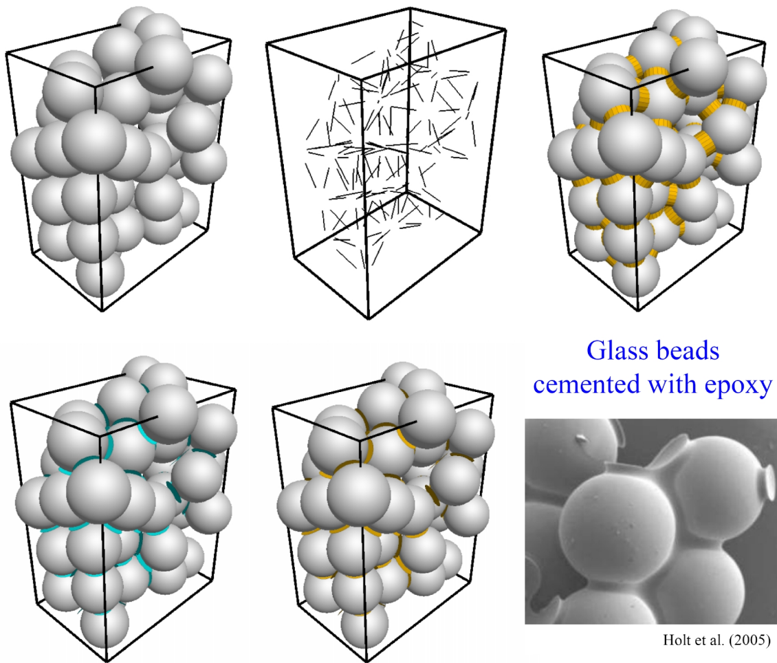
Figure 17 Microstructural plot sets for bonded materials with the same initial packing showing (clockwise from upper left): microstructural box and grains in the box (grey); contact-bonded material with contact bonds in the box; parallel-bonded material with parallel-bond cement (gold, 50% size) and parallel-bond interfaces (gold, 50% size); and flat-jointed material with flat-jointed interfaces (blue, 50% size).
