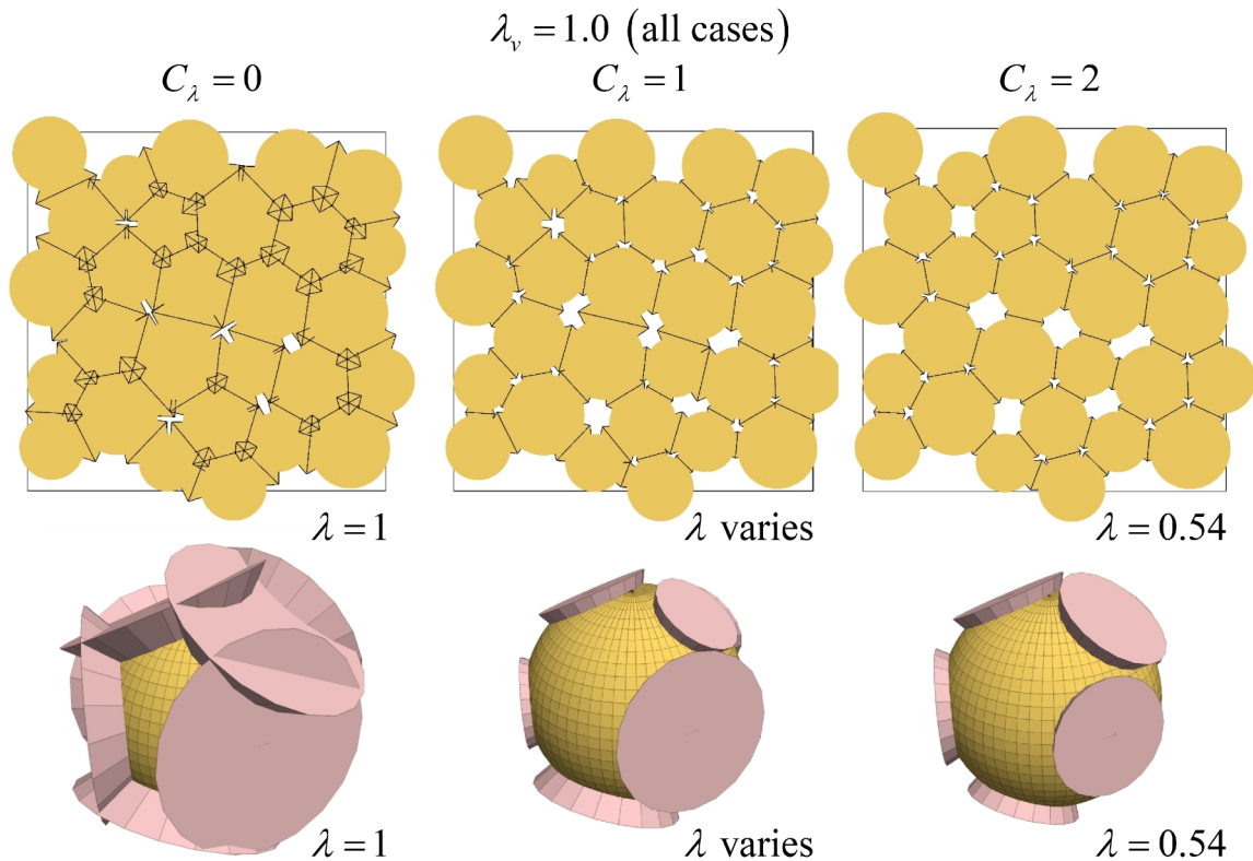
Figure 14 The three types of flat-jointed microstructures produced by the material-modeling support package. The left-most images have invalid microstructures, while the middle and right images have valid microstructures. Only a single faced grain is shown for the 3D case (bottom).
