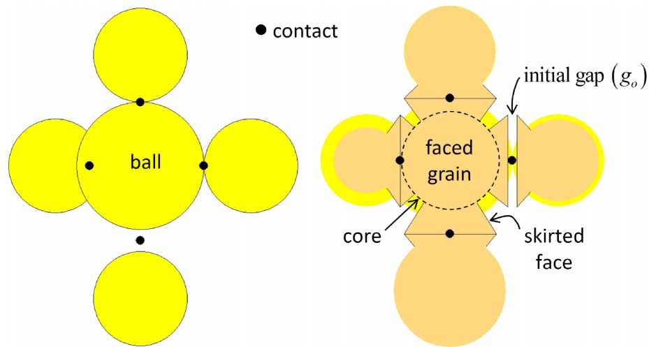
Figure 11 Creation of faced grains showing packed ball assembly (left) and initial faced-grain assembly (right). (From Fig. 2 of Itasca [2019] 21 .)
