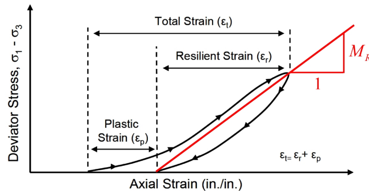
Figure 30 Response of granular material subjected to triaxial loading, and measurement of resilient modulus. (From Fig. 1 of Buchanan [2007].)
