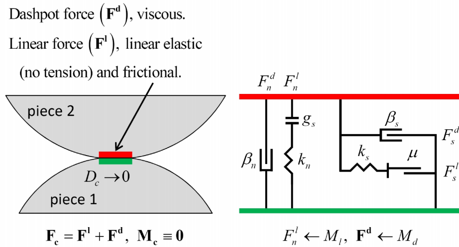
Figure 4 Behavior and rheological components of the linear model. (From Fig. 1 of Itasca [2019] 11 .)
