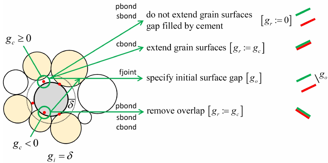
Figure 27 Setting final material properties of bonded materials to establish reference surfaces that do not overlap (contact-bonded, parallel-bonded, soft-bonded and flat-jointed materials denoted by cbond, pbond, sbond and fjoint, respectively).
