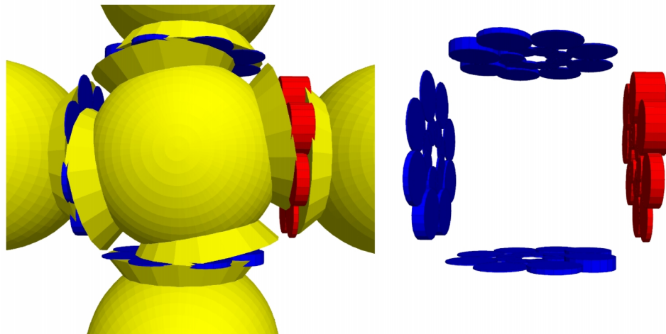
Figure 20 Crack and faced grain plot sets in 3D showing cracks, with crack thickness equal to gap, and cracks colored red/blue for tensile/shear failure.
